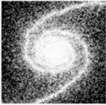
Milky Way
